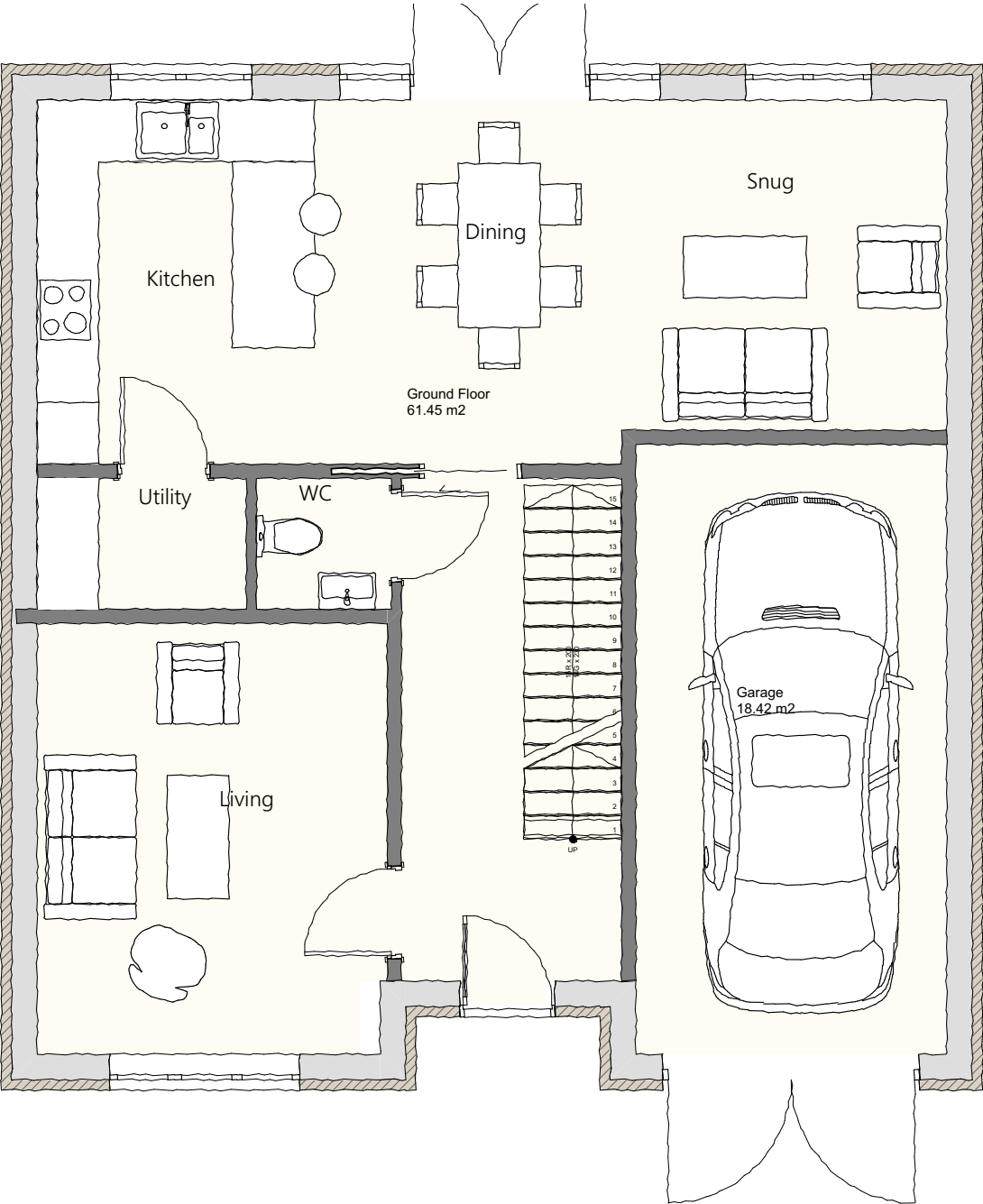
0. Ground Floor 1:50
