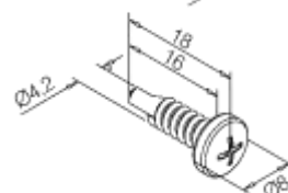
Self drilling cross recessed pan head screw, wrought iron effect Blechschrabe selbstschneidend, Schmiedeeisen-Effekt Vis autotaraudeuse, aspect fer forgé Zelfborende metaalschroef, smeedijzer look Art.Nr. 19.0010.000.38
