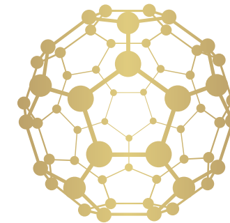
Fullerene C 60
